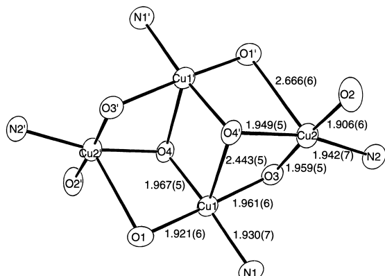
Fig. 10. Core structure of [\text{Cu}_4(\text{bzacpro})_2(\text{C}_2\text{H}_5\text{O})_2] ( 2 ).
