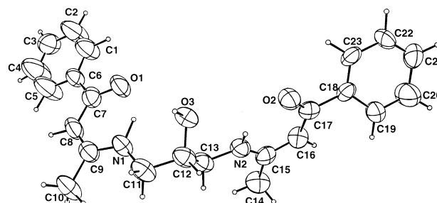
Fig. 1. ORTEP drawing of the structure of H_3bzacpro , showing the atom-labeling scheme. Thermal ellipsoids are at the 50% probability.
