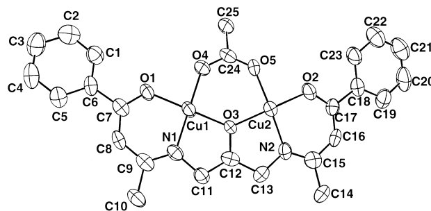
Fig. 4. ORTEP drawing of the structure of [Cu_2(bzacpro)(CH_3CO_2)] ( 1 ) showing the 35% probability thermal ellipsoids and atom labeling scheme. Hydrogen atoms are omitted for clarity.
