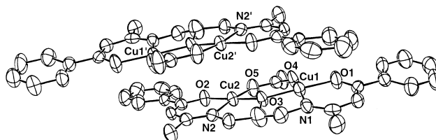
Fig. 5. View of the stacking feature of [Cu_2(bzacpro)(CH_3CO_2)] ( 1 ).
