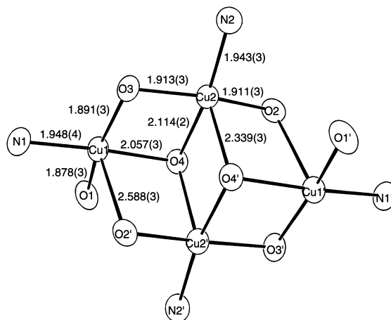
Fig. 8. Core structure of [\text{Cu}_4(\text{bzacpen})_2(\text{CH}_3\text{CO}_2)_2] ( 5 ).
