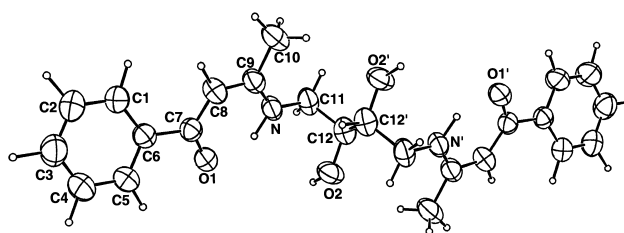
Fig. 2. ORTEP drawing of the structure of H_3bzacbu , showing the atom-labeling scheme. Thermal ellipsoids are at the 50% probability.
