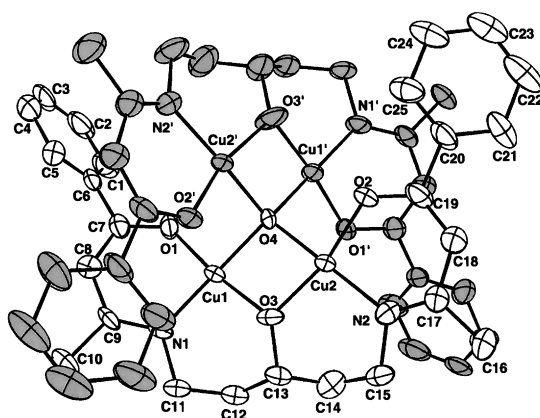
Fig. 13. ORTEP drawing of the structure of [\text{Cu}_4(\text{bzacpen})_2\text{O}]\cdot\text{H}_2\text{O} ( 6 ) showing the 35% probability thermal ellipsoids and atom labeling scheme. Hydrogen atoms and solvent molecule are omitted for clarity. Primed and unprimed atoms are related by the C_2 axis.
