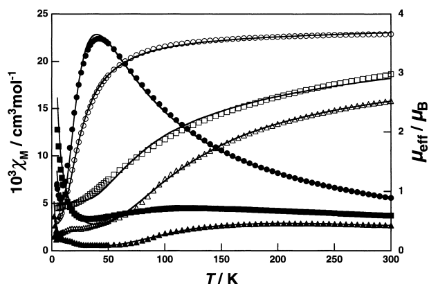
Fig. 16. Magnetic susceptibility data (●, ▲, ■) and effective magnetic moments (○, △, □) of [\text{Cu}_4(\text{bzacpro})_2(\text{C}_2\text{H}_5\text{O})_2] ( 2 ) [\text{Cu}_4(\text{bzacpen})_2(\text{CH}_3\text{CO}_2)_2] ( 5 ) and [\text{Cu}_4(\text{bzacpen})_2\text{O}] \cdot \text{H}_2\text{O} ( 6 ). The solid lines show the best fit obtained (see text).
