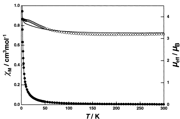
Fig. 17. Magnetic susceptibility data (●) and effective magnetic moment (○) of [\text{Cu}_4(\text{bzacbu})_2(\text{CH}_3\text{O})_2] ( 4 ). The solid lines show the best fit obtained (see text).
