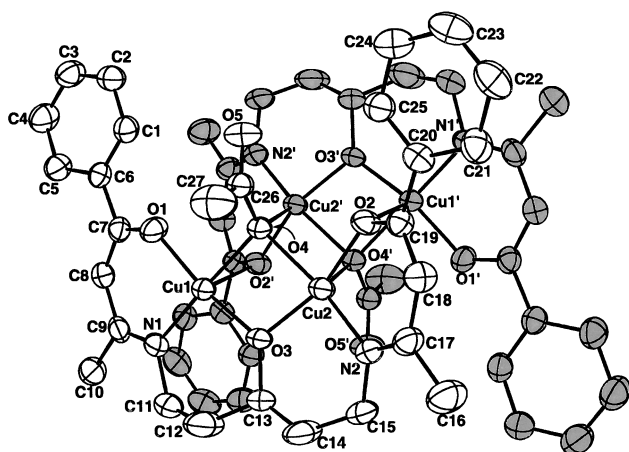
Fig. 7. ORTEP drawing of the structure of [\text{Cu}_4(\text{bzacpen})_2(\text{CH}_3\text{CO}_2)_2] ( 5 ) showing the 50% probability thermal ellipsoids and atom labeling scheme. Hydrogen atoms are omitted for clarity.
