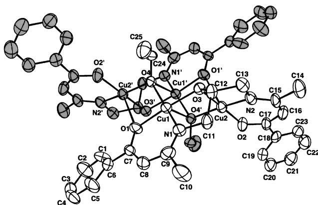
Fig. 9. ORTEP drawing of the structure of [\text{Cu}_4(\text{bzacpro})_2(\text{C}_2\text{H}_5\text{O})_2] ( 2 ) showing the 35% probability thermal ellipsoids and atom labeling scheme. Hydrogen atoms are omitted for clarity.
