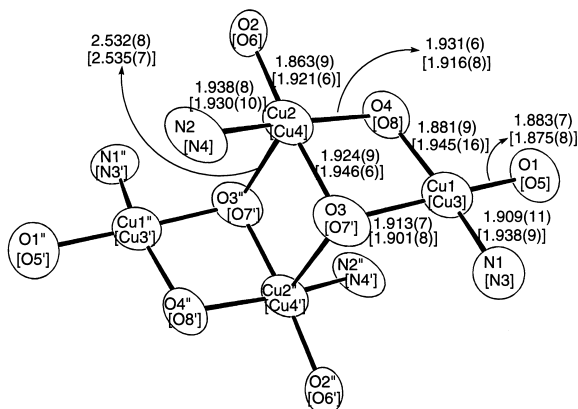
Fig. 12. Core structure of [\text{Cu}_4(\text{bzacbu})_2(\text{CH}_3\text{O})_2] ( 4 ).
