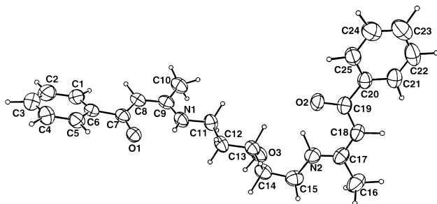
Fig. 3. ORTEP drawing of the structure of H_3bzacpen , showing the atom-labeling scheme. Thermal ellipsoids are at the 50% probability.
