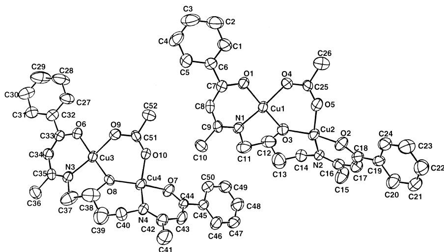
Fig. 6. ORTEP drawing of the structure of [\text{Cu}_2(\text{bzacbu})(\text{CH}_3\text{CO}_2)] ( 3 ) showing the 35% probability thermal ellipsoids and atom labeling scheme. Hydrogen atoms are omitted for clarity.
