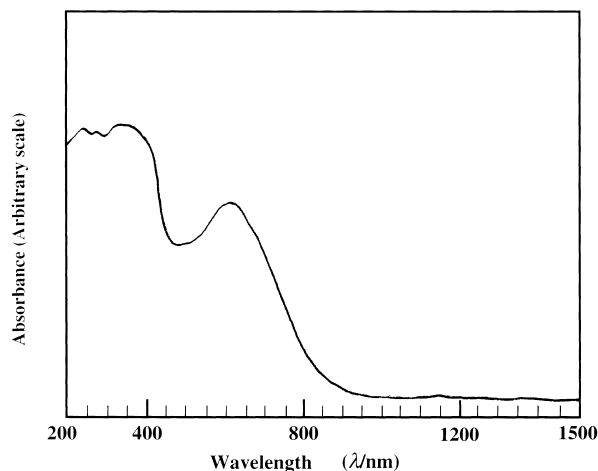
Fig. 14. Diffuse reflectance spectrum of [\text{Cu}_2(\text{bzacpro})(\text{CH}_3\text{CO}_2)] ( 1 ).
