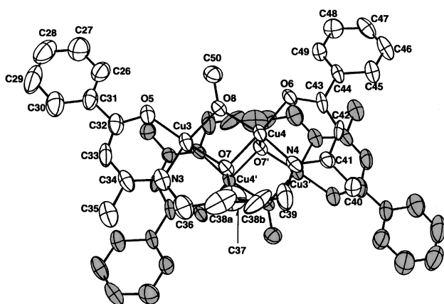
Fig. 11. ORTEP drawing of the structure (molecule b) of [\text{Cu}_4(\text{bzacbu})_2(\text{CH}_3\text{O})_2] ( 4 ) showing the 35% probability thermal ellipsoids and atom labeling scheme. Hydrogen atoms are omitted for clarity. Primed and unprimed atoms are related by the inversion.
