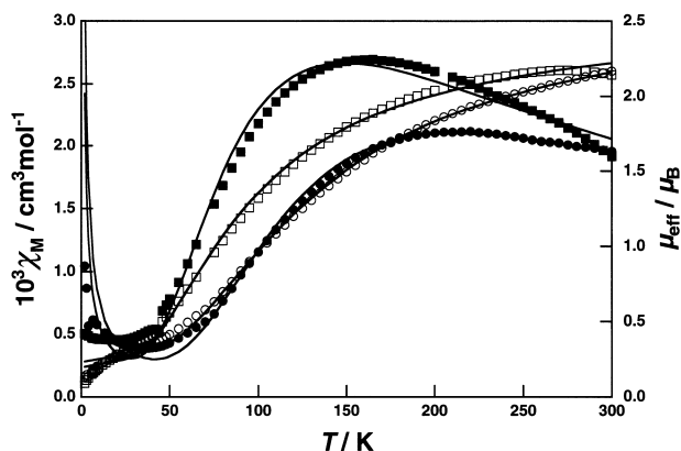
Fig. 15. Magnetic susceptibility data (■, ●) and effective magnetic moments (□, ○) of [\text{Cu}_2(\text{bzacpro})(\text{CH}_3\text{CO}_2)] ( 1 ) and [\text{Cu}_2(\text{bzacbu})(\text{CH}_3\text{CO}_2)] ( 3 ). The solid lines show the best fit obtained (see text).
