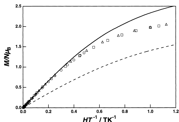
Fig. 18. Field dependence of the magnetization: experimental data for [\text{Cu}_4(\text{bzacbu})_2(\text{CH}_3\text{O})_2] ( 4 ) at 4 (△), 4.5 (□), and 10 K (○); theoretical curves for S = 3/2 (—) and S = 1 (---) spin states ( g = 2.0 ).
